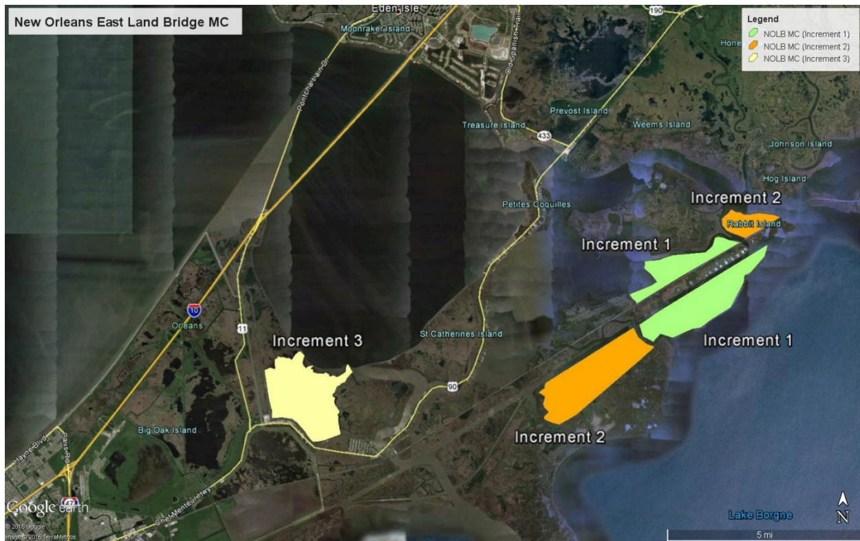
Figure 18. New Orleans East Land Bridge Project
